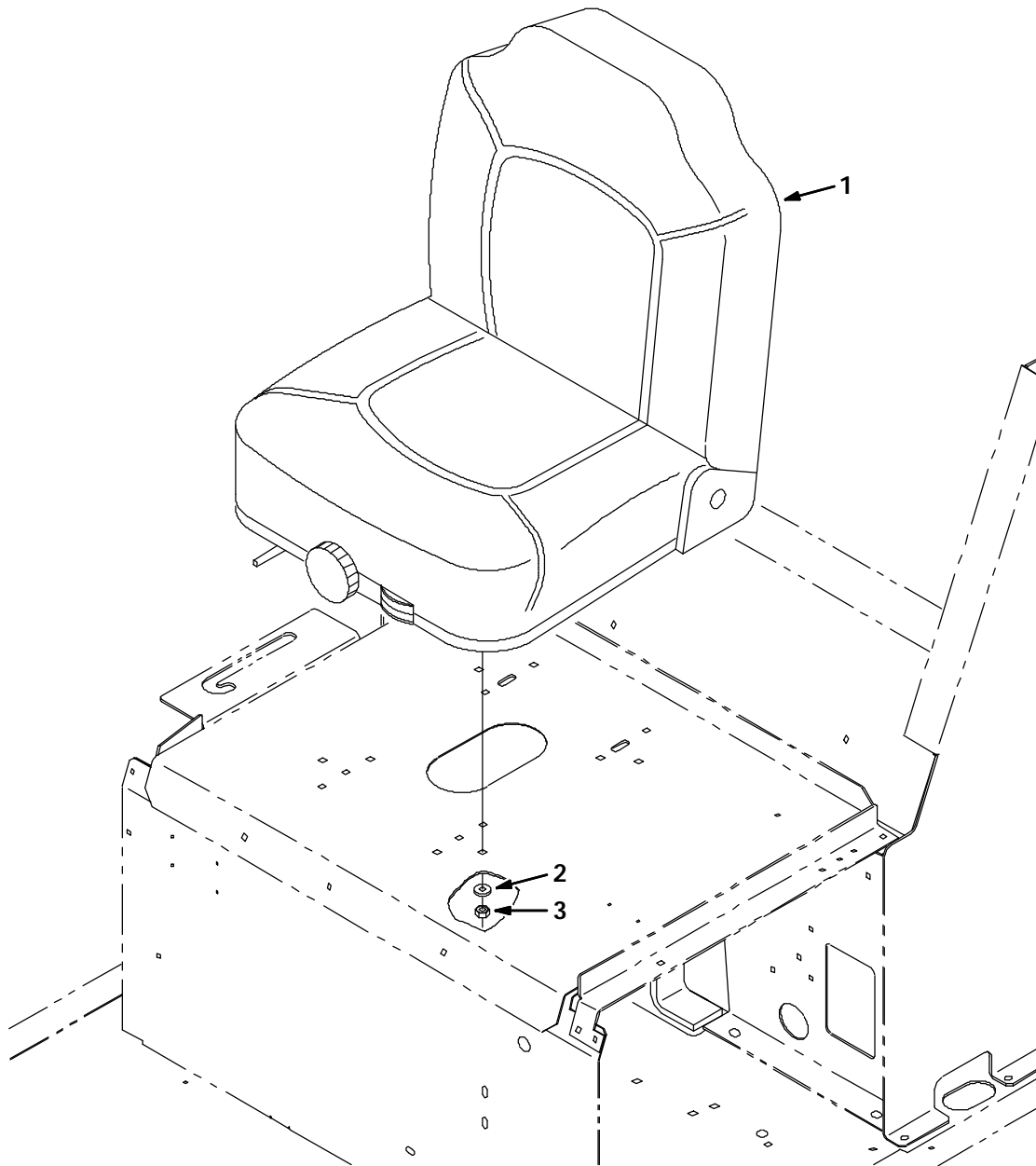
FIG. 1 - SUSPENSION SEAT INSTALLATION
